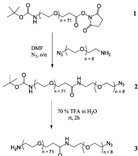
Scheme 2. Synthesis of H 2 N-PEG-N 3 by Reacting NHS-Activated PEG Chains with Amine-Terminated Octaethylene Glycol-Azide Followed by BOC Deprotection
